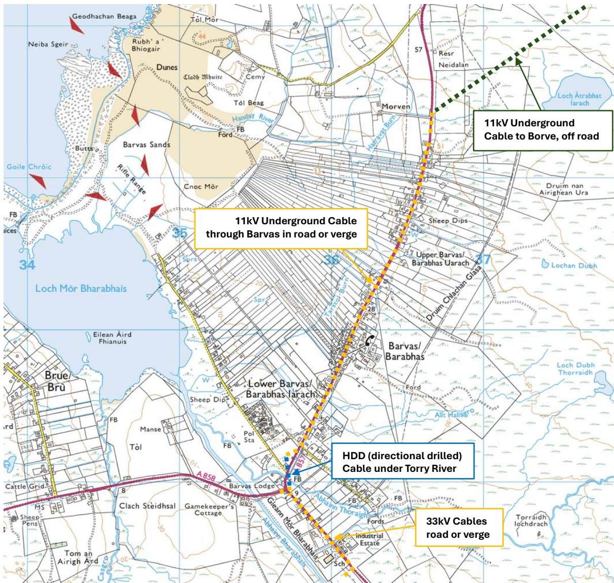
33kV / 11kV Cable – Barvas to Borve
