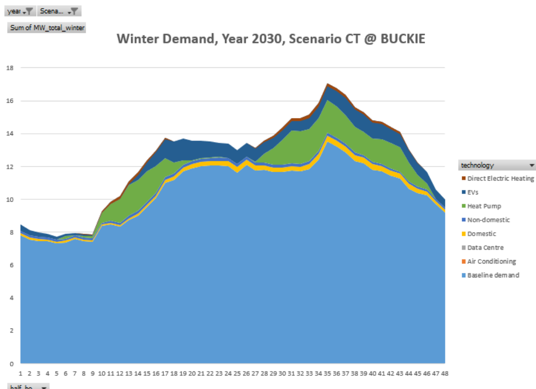
Figure 6: Future Substation Demand Profile
