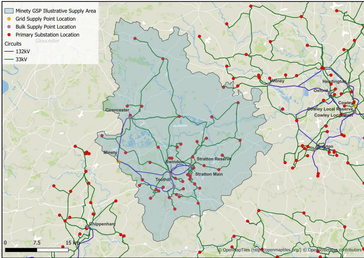
Figure 5 Current network topology of Minety GSP
