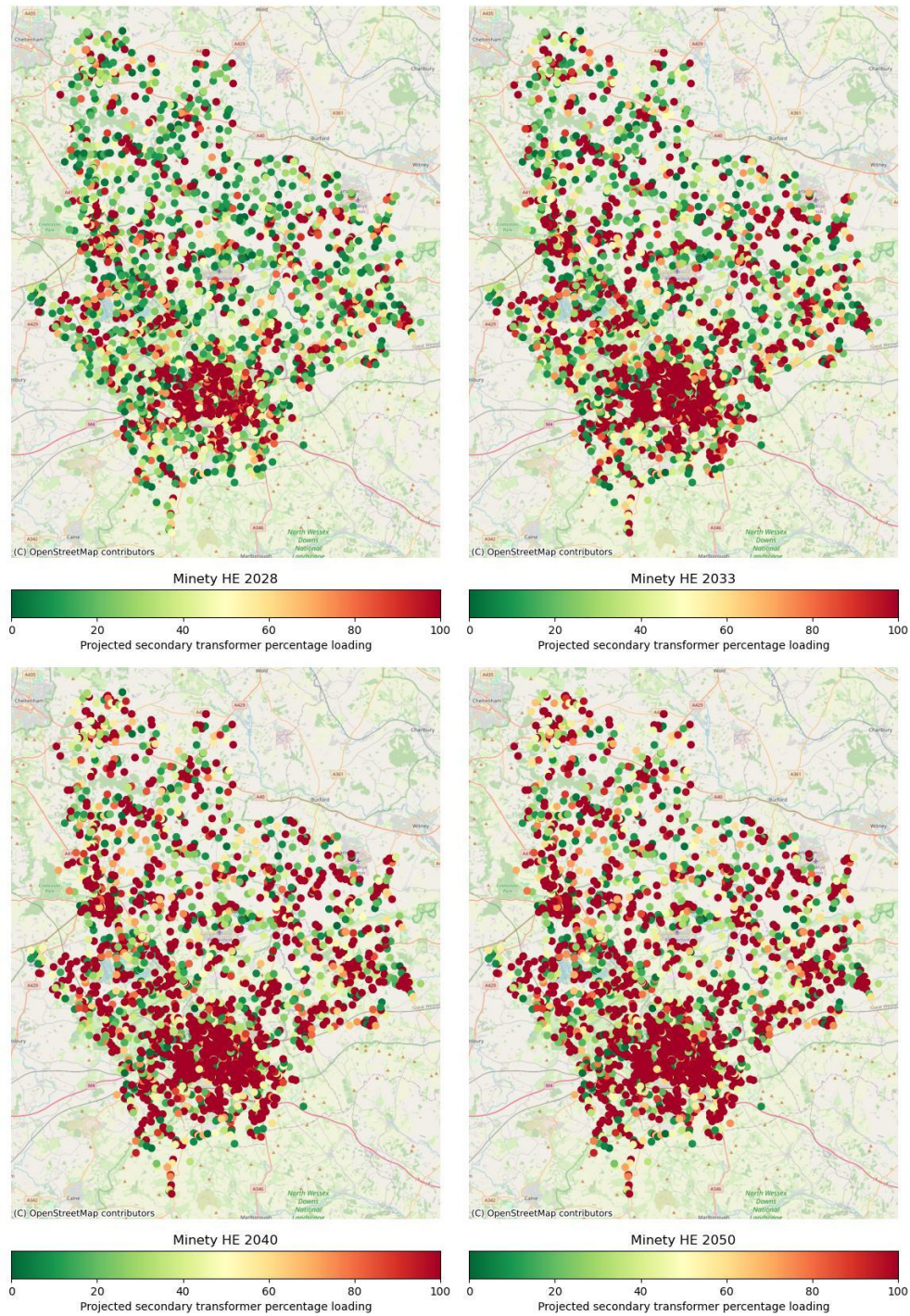
Figure 32 Minity GSP - HV/LV Spatial Plan – Hydrogen Evolution
