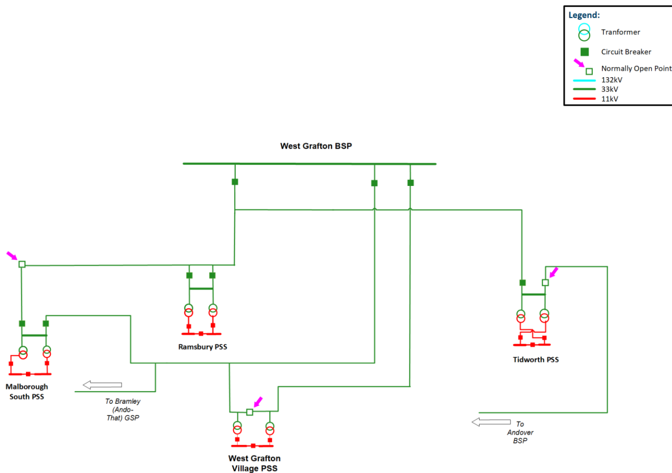
Figure 22: West Grafton BSP - Existing network schematic
