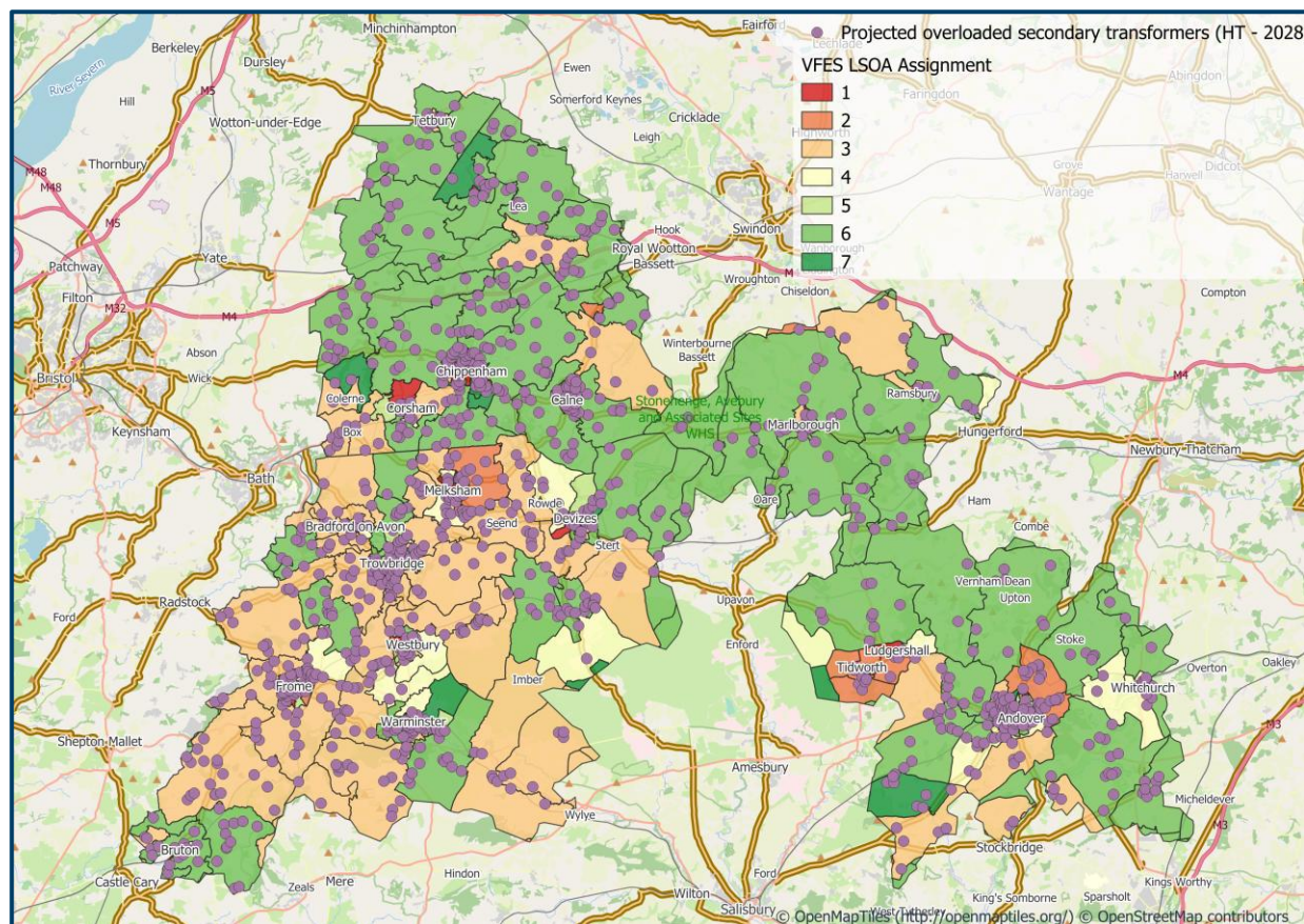
Figure 4: Melksham GSP VFES Output with secondary transformer overlay.
