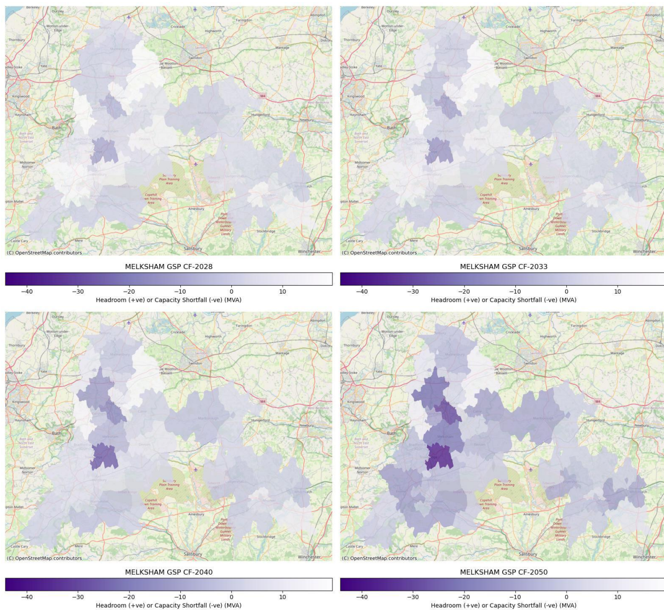
Figure 27: Melksham GSP - EHV/HV Spatial Plan - Counterfactual
